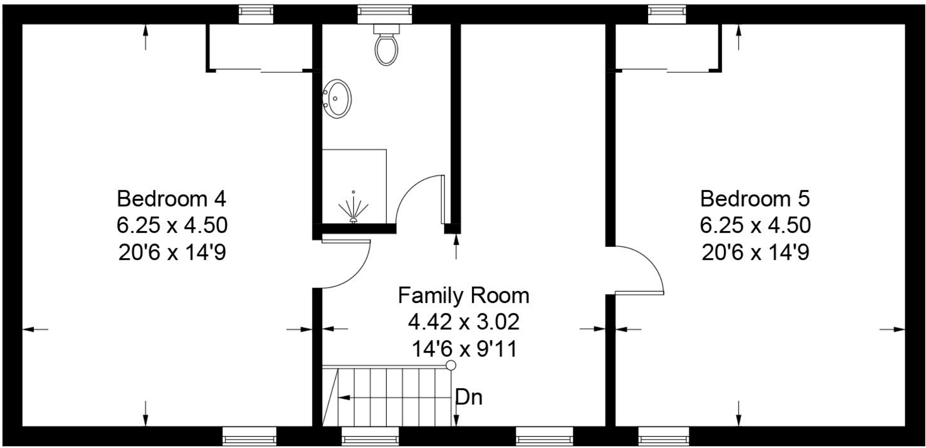
First Floor
